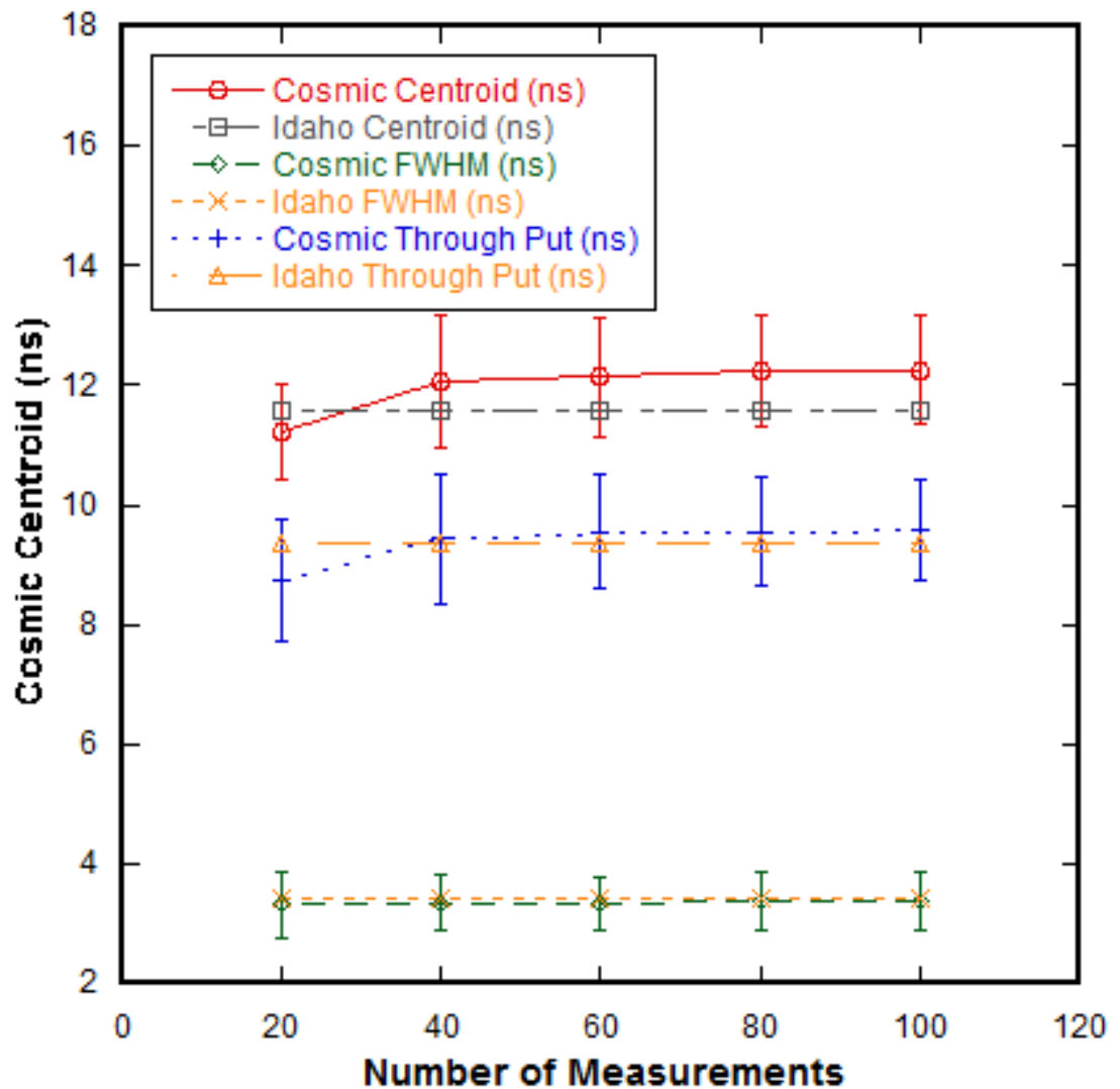
Figure 31: Analytical Results from Taking Additional Measurements on D1 at -2500V
