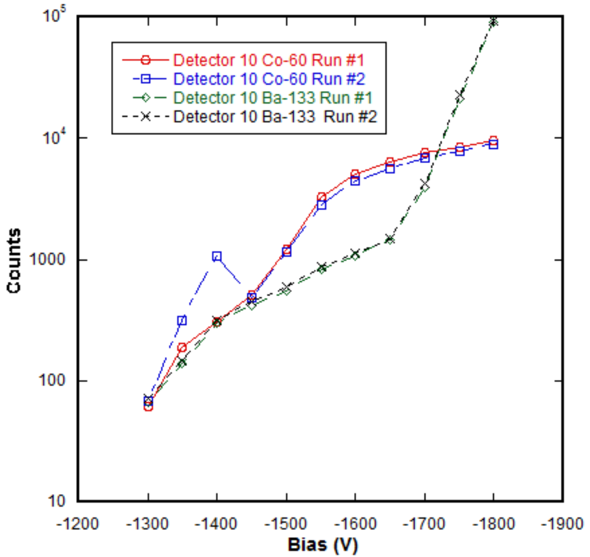
Figure 7: Cosmic Detector 10 Co-60 and Ba-133 Counting Plateaus
